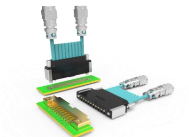
Figure 9: 8 channel coreHC to 1.85mm cable
